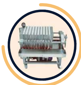
SH: PRF - 500 (Plate Ring Filter)
